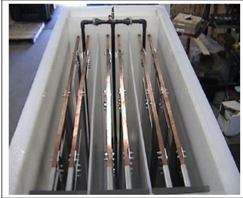
OZOLECTROCLEAN REACTOR Open Type
